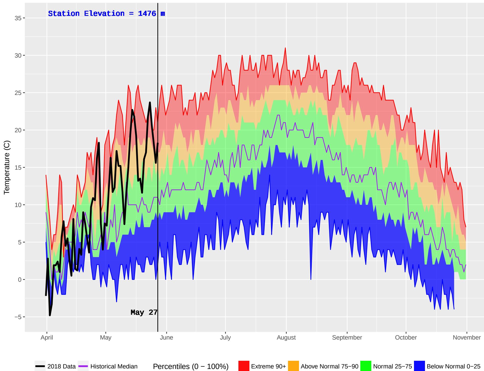
BRENDA MINES (283) : Historical (1977–2016) and Current (2018) Noon Temperature
